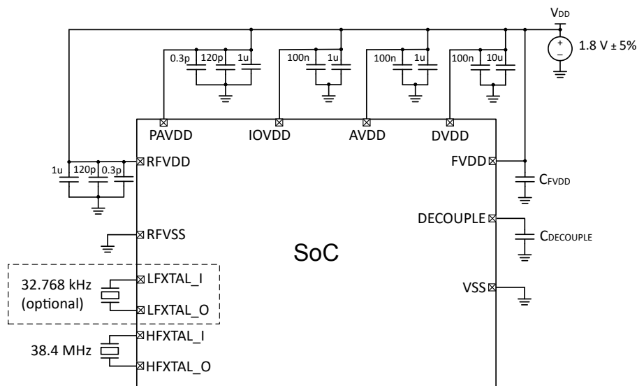
Figure 5.2. Single Supply ( 1.8 \text{ V} \pm 5\% )
